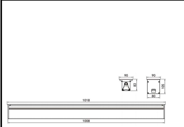
Dimension diagram
